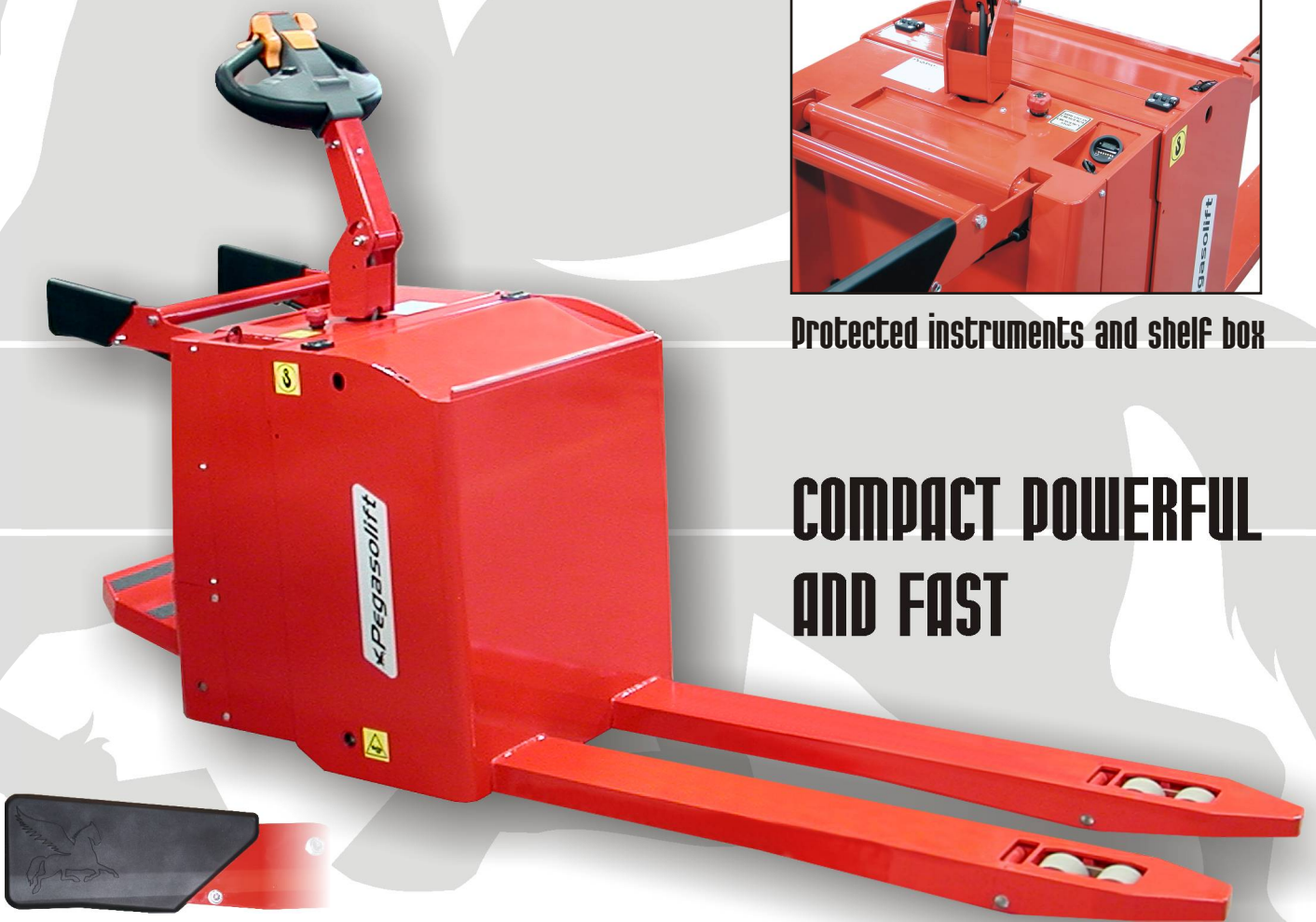
Side arms with rubber protection and platform retractable integrated in the rear cover
